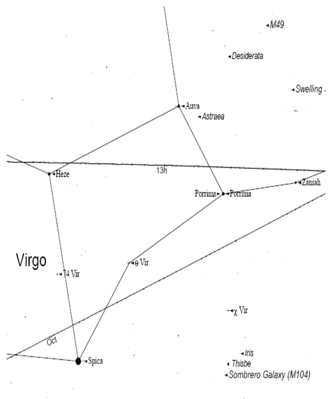
Finder Chart for M104
